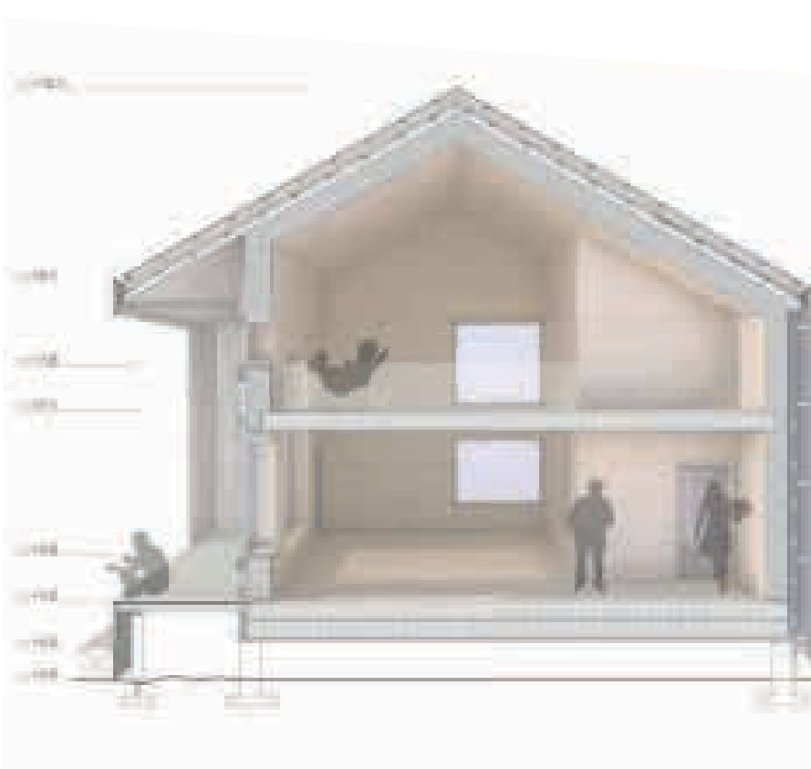
Fasadskärning
